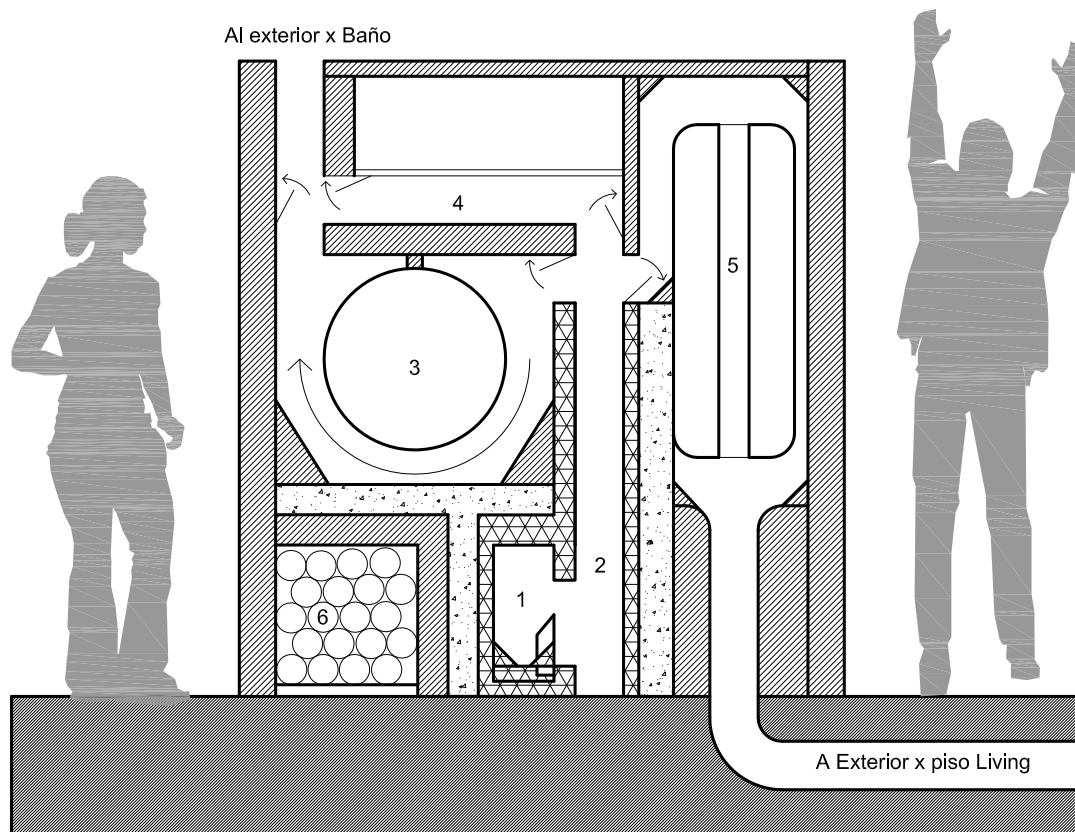
Vista Frontal
